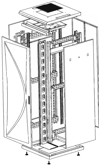
Explode View
