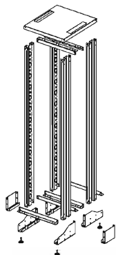
Explode View
